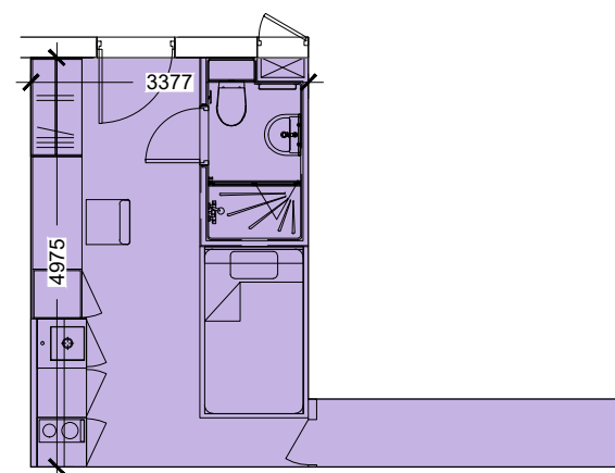
SINGLE BEDROOM Type 02K
