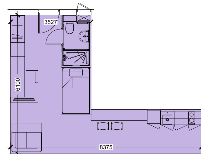
SINGLE BEDROOM Type 02G
