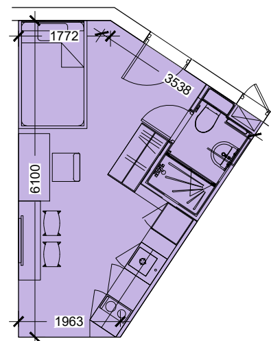
SINGLE BEDROOM Type 02J
