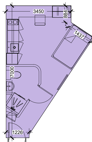
SINGLE BEDROOM Type 02H
