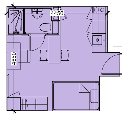
SINGLE BEDROOM Type 02F
