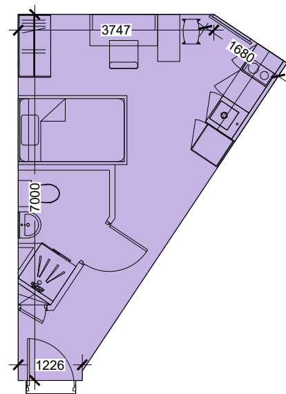
SINGLE BEDROOM Type 02D
