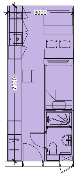
SINGLE BEDROOM Type 02A 21.0 sq.m.
