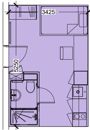
SINGLE BEDROOM Type 01N 18 sq.m.
