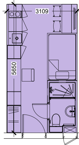
SINGLE BEDROOM Type 01W 17.6 sq.m.
