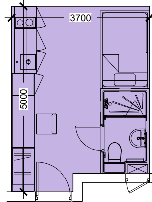
SINGLE BEDROOM Type 01P 17.4 sq.m.
