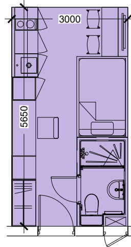
SINGLE BEDROOM Type 01U 16.9 sq.m.
