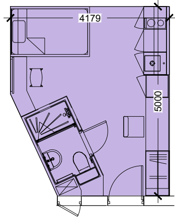
SINGLE BEDROOM Type 01O 19.2 sq.m.
