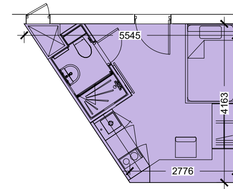
SINGLE BEDROOM Type 01S 17.3 sq.m.
