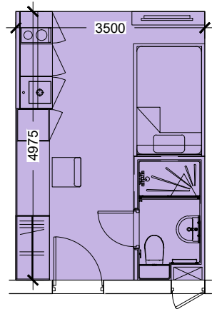
SINGLE BEDROOM Type 01T 18.2 sq.m.
