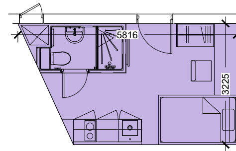
SINGLE BEDROOM Type 01R 16.4 sq.m.
