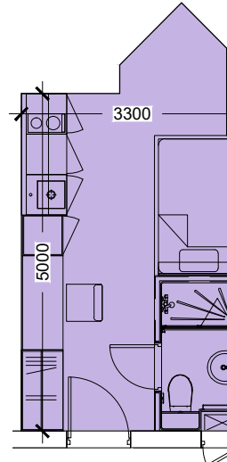
SINGLE BEDROOM Type 01F 18.1 sq.m.
