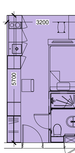
SINGLE BEDROOM Type 01D 18.2 sq.m.
