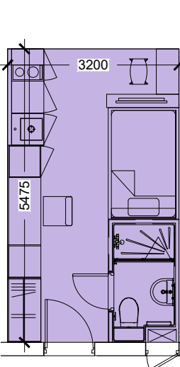
SINGLE BEDROOM Type 01C 17.5 sq.m.
