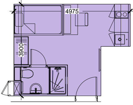
SINGLE BEDROOM Type 01J 16.8 sq.m.
