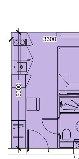
SINGLE BEDROOM Type 01E 16.5 sq.m.
