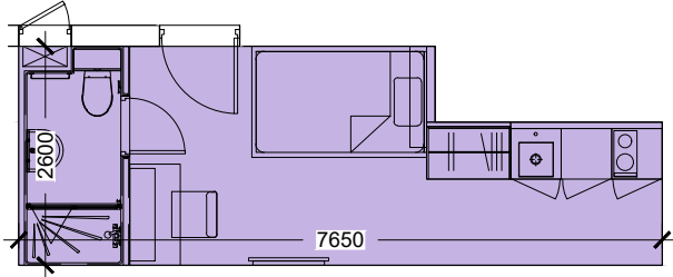
SINGLE BEDROOM Type 01K 17.5 sq.m.
