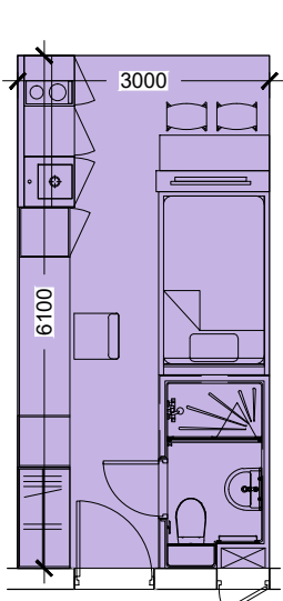
SINGLE BEDROOM Type 01H 18.3 sq.m.
