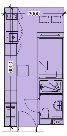
SINGLE BEDROOM Type 01A 17.8 sq.m.
