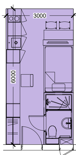
SINGLE BEDROOM Type 01 18 sq.m.
