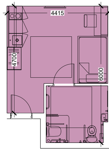
ACCESSIBLE BEDROOM Type 03 23.7 sq.m.
