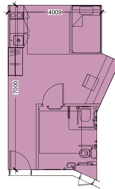
ACCESSIBLE BEDROOM Type 03B 28.5 sq.m.
