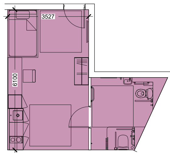
ACCESSIBLE BEDROOM Type 03A 30.1 sq.m.
